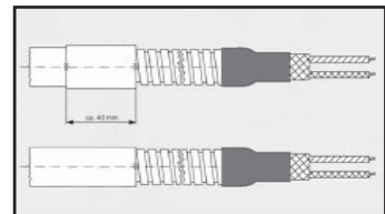
Armor cable
