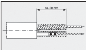
Crimped outside heater
