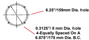
Mounting Pattern
