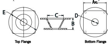
Machine Mount Adapter (Included with MM mode[s])
